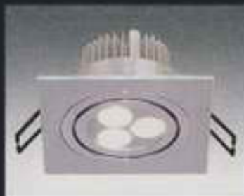
Item: TS TH5-3W Size: 92×92×47mm 3×1W LED 220V with Driver
