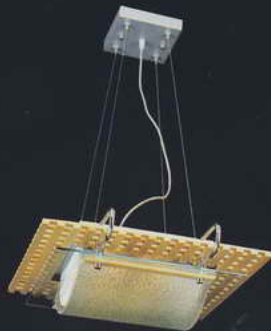
Item: TS P0003-4B Size: 55×46.5×12cm 4×E27 - 220V
